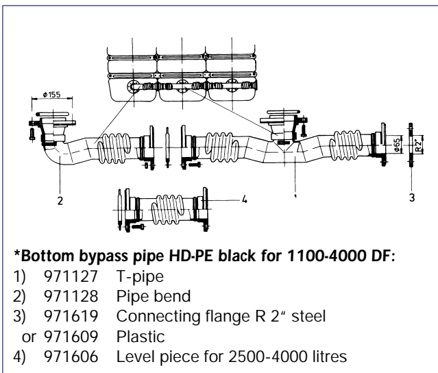
Expandable tank group with bottom bypass pipe.
