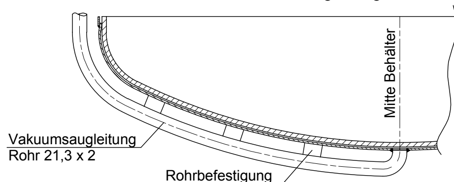
Detail "U"
