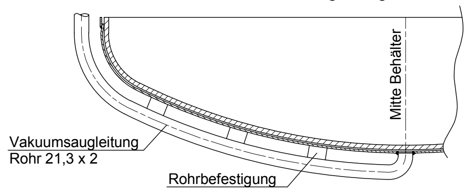
Detail "U"
