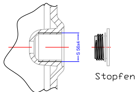
Detail Z
