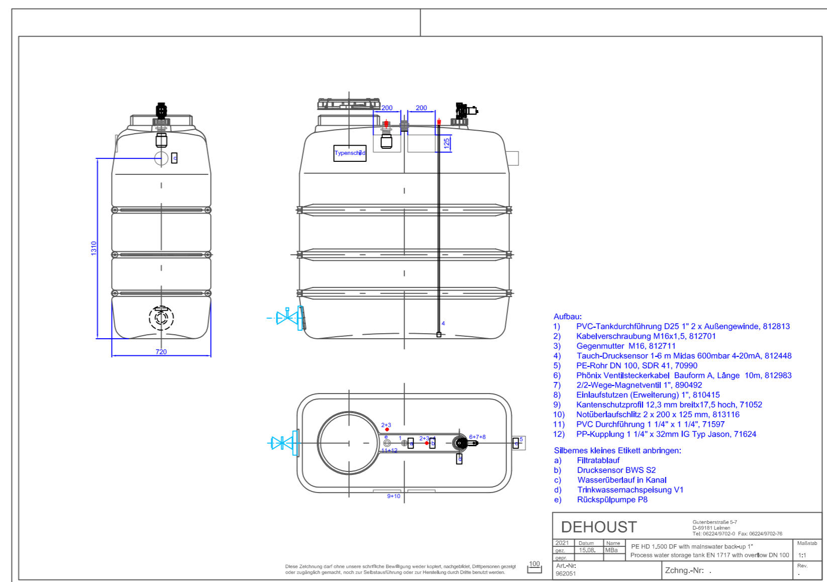
Process water storage tank PE HD 1.500 DF
