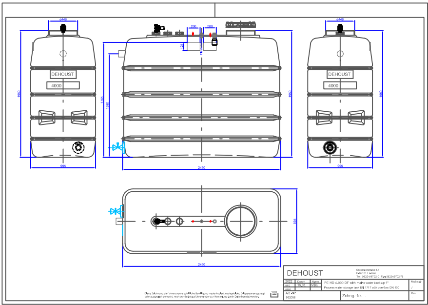
Process water storage tank PE HD 4.000 DF
