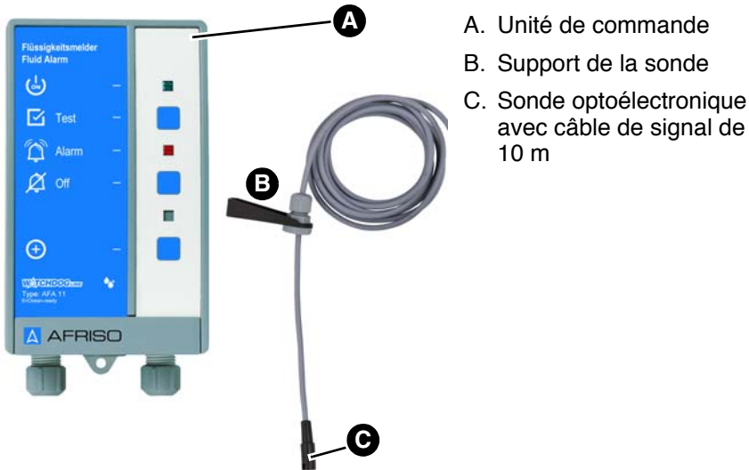
Figure 3: Composants fournis
